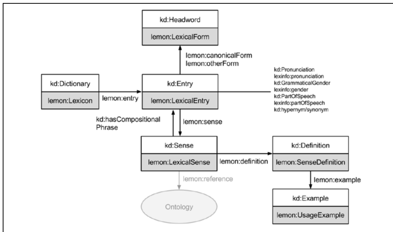
Figure 6: Mapping KD's XML elements and lemon resources (excluding the greyed out Ontology part)
